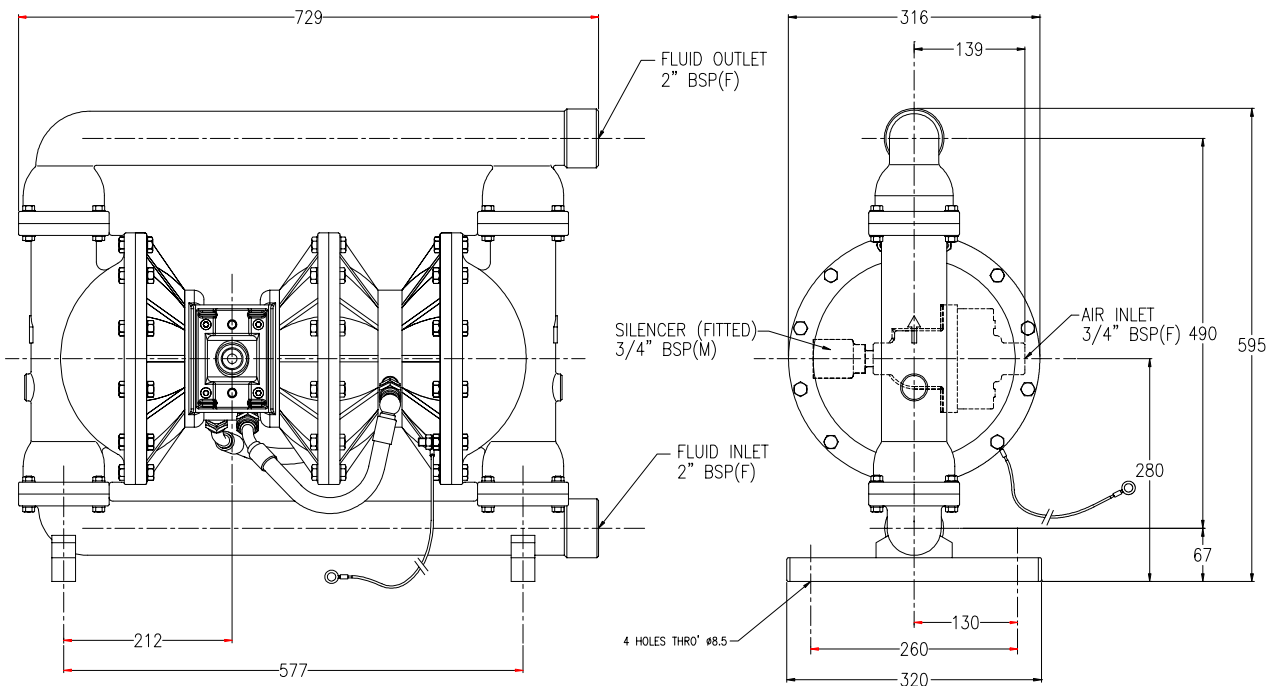
General Assembly B50 / X5002 Full Flow 2:1 Pump :- All dimensions +/- 3mm
